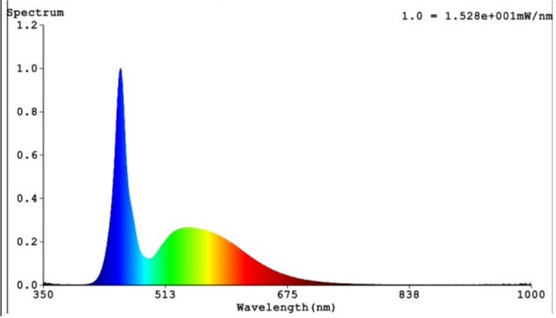
Spectral power distribution in the range 250 nm to 800 nm, at full-load
